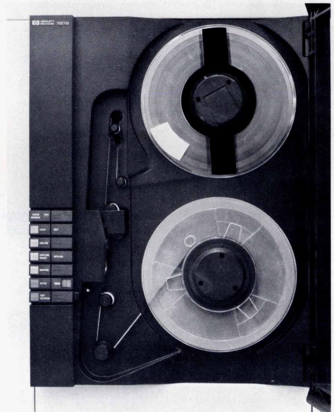
Fig 1. Designed to back up computer systems with large amounts of on-line disc storage, HP's newest half-inch tape drive, the HP 7978A, features high performance and increased reliability for a low cost. This streaming tape drive uses both 6250 GCR and 1600 PE storage formats.
